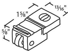
#018-29 Nylon Metal 9/16" Dia. Roller
