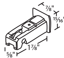
#018-68 Aluminum Grooved Nylon 1/2" Dia. Rollers
