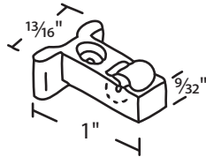
#018-649 Metal 3/8" Dia. Roller
