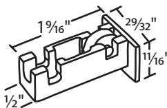
#018-77 Nylon Metal 1/2" Dia. Roller
