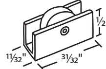
#018-613 Nylon 9/16" Dia. Roller #018-675 Metal 9/16" Dia. Roller
