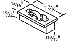
#018-680 Nylon 9/16" Dia. Roller
