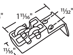
#018-618 Nylon 15/32" Dia. Roller
