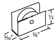
#018-68 Aluminum Grooved Nylon 1/2" Dia. Rollers
