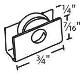
#018-676 Metal 1 7/32" Dia. Roller
