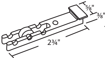
#018-658 Nylon 7/16" Dia. Roller
