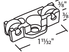
#018-83 Aluminum Nylon 15/32" Dia. Roller
