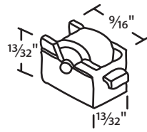
#018-47 Nylon Steel 7/16" Dia. Roller
