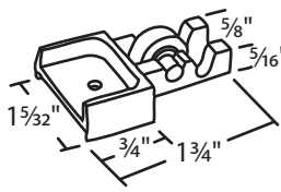
#018-644 Metal 5/8" Dia. Roller
