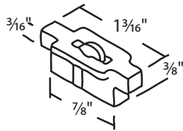
#018-87B Nylon Brass 7/16" Dia. Roller
