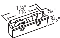
#018-86 Nylon Metal 1/2" Dia. Roller
