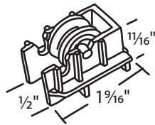
#018-646 Nylon 5/8" Dia. Roller
