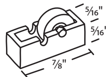
#018-90 Nylon Metal 15/32" Dia. Roller
