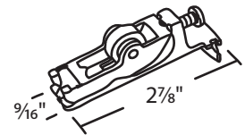
#018-650 Metal Nylon 5/8" Dia. Roller
