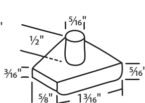
#09-79 Aluminum Sold in Sets
