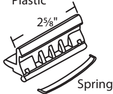
#02-161 Black #02-161W White Plastic
