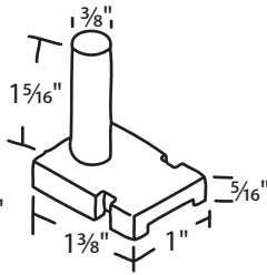
#09-79 Aluminum Sold in Sets
