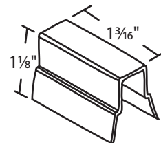
#05-164 Double Hung Bracket Installation Bracket
