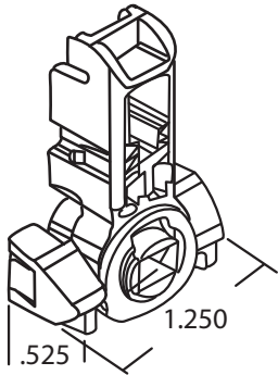
T-Lock/Molded Spring
