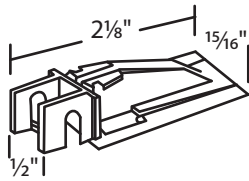
#02-0563 Old Style Security, Jones
