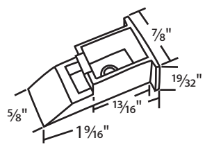
#02-838 Black LH & RH Set
