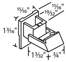
#02-838 Black LH & RH Set
