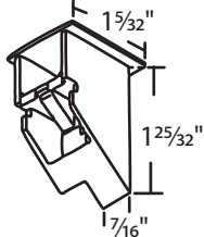
#02-1880 RH & LH Set
