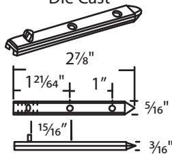
#01-32-30 Tie-In Die Cast
