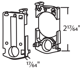
#01-32-30 Tie-In Die Cast
