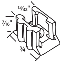
#094-10 Sash Clips Howard
