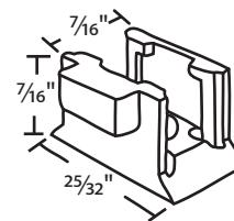
#094-13 Sash Clip Portalume
