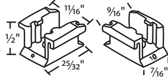
#094-20 LH/RH Set Sash Clips Airmaster
