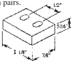
#09-850 Aluminum
