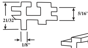
Pivot Bar Holder #025-25 Black Length: 2 15/16"
