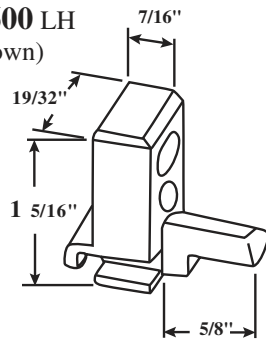
#020-36 RH #020-37 LH (RH Shown)
