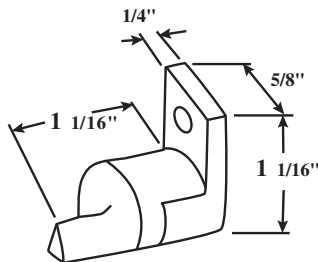
#02-2601 RH #02-2600 LH (LH Shown)
