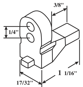
#020-36 RH #020-37 LH (RH Shown)
