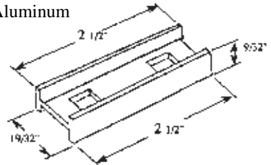
#02-626 Sash Guide-Use with #01-12 Bracket
