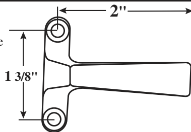
#03-100 Pull Handle White Bronze
