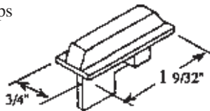
#02-5604 White #02-5605 Black Top Sash Dust Caps
