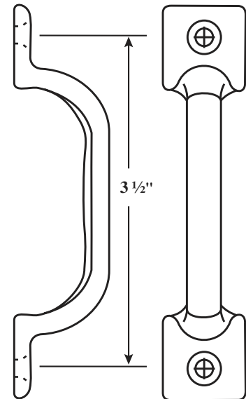
#03-150 Pull Handle White Bronze
