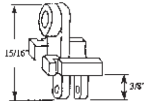
#02-626 Sash Guide-Use with #01-12 Bracket
