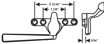
#023-298 RH Shown #023-299 LH White Bronze
